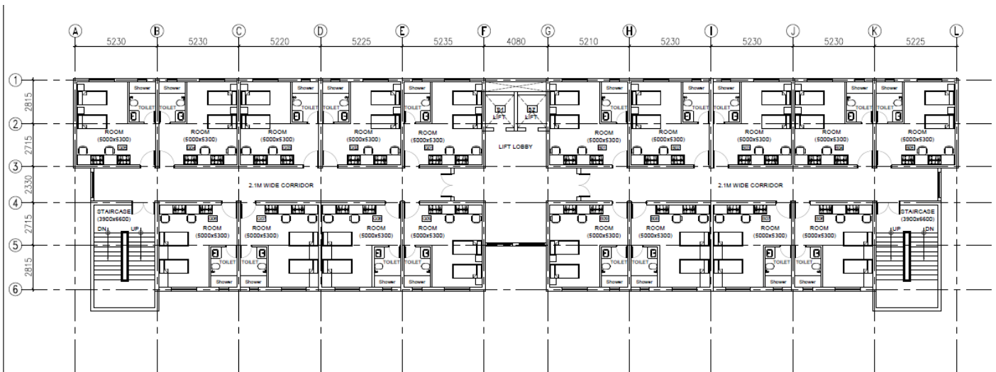
TYPICAL FLOOR PLAN (SECOND & THIRD)
